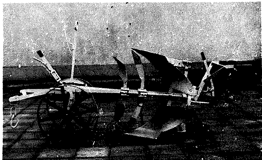
Herteant Reversible Plow LEIE-9 Willem Herteant
