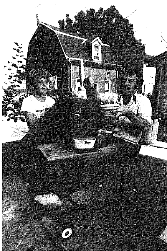
The Miller Boy Mill seen here has been modified from electric to pedal power. The pedal power unit, called the Energy Cycle, is a product of Rodale Resources Division, Emmaus, Pa.
