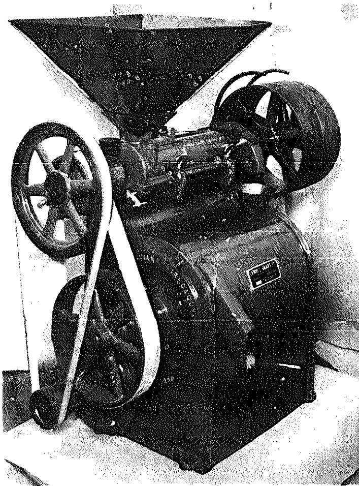
Grantex Rice Huller Lewis C. Grant, Ltd.
