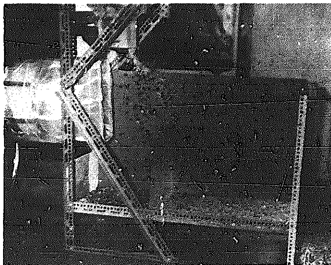
A demonstration of the pedal winnower in action. Notice that the larger, heavier matter falls first and that the lighter chaff is blown far away as the grain mixture falls from a hopper above. Dr. B. N. Ghosh
