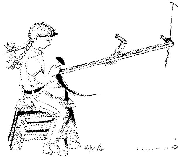
10. A simple arrangement for holding the scythe when peening.
