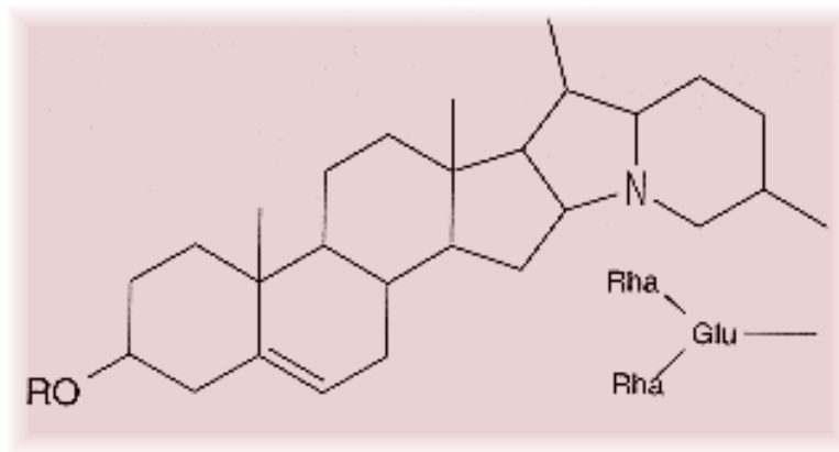
nitrate solanine
