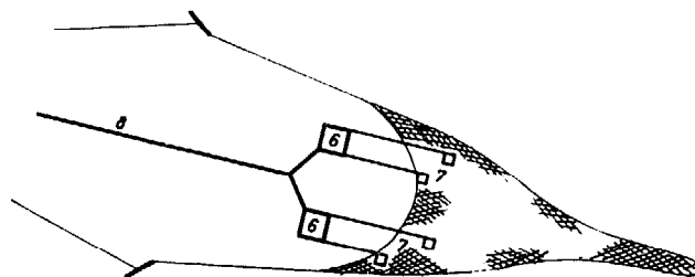
Fig 500 Sketch of electrical trawling method, according to C O Kreuzer (Scharfe, 1965) 1. Diesel engine 2. Generator 3. Electrical impulse transmitter 4. Transformer 5. Control apparatus for impulse transmitter 6. Impulse transformer 7. Electrodes 8. Warps.
