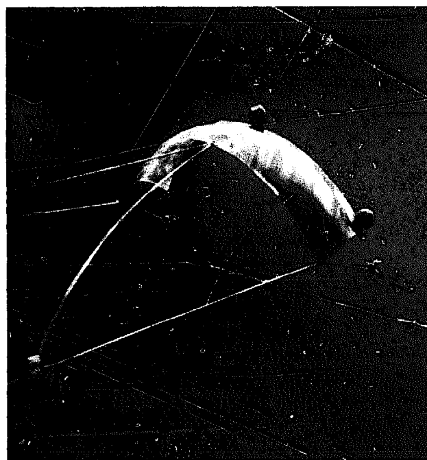
Fig 486 Sailkite for a rope trawl. (Photo: W Horn, 1980).
