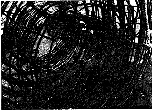
Fig 389 Australian rock lobster pot made of wood and wire in Tasmania. The mesh of the base is of very stiff wire and is therefore made by simple twisting, without knotting.
