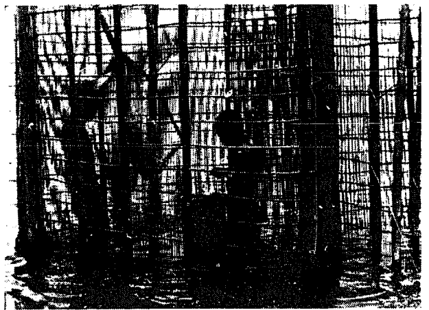
Fig 348 In this large bamboo weir of the Philippines a slit, as a non-returning device (see above), gives entrance to the catching room from which the catch is secured with scoop nets at low tide (see below). (1960)
