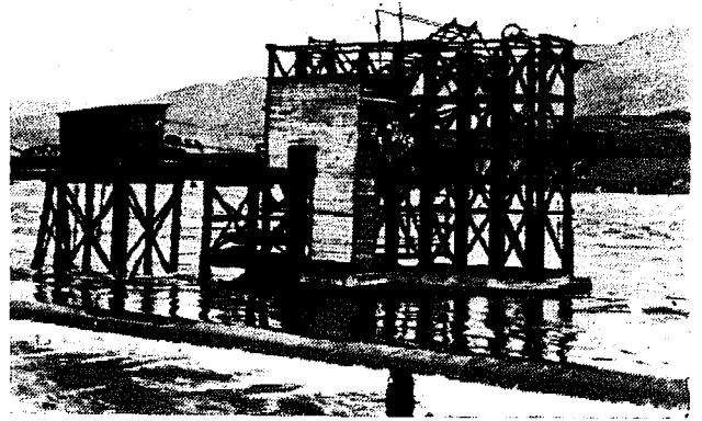
Fig 642 A stationary wheel in the Celilo area, Oregon, USA. ( Photo: Donaldson. )
