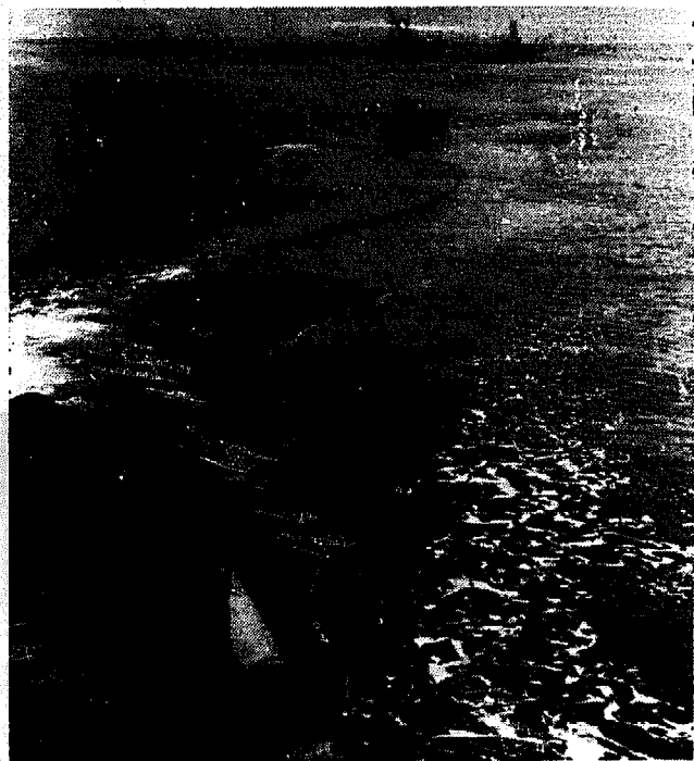
Fig 567 Shooting a Peruvian purse seine with one boat and a skiff. (Photo: Brandhorst)
