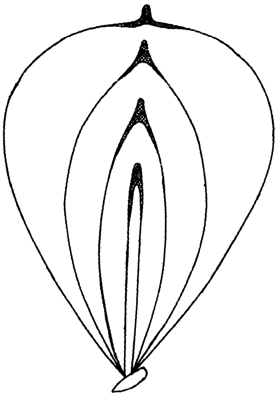
Fig 552 Expected shape of a Danish seine during hauling, without, and with, floating otter boards. (According to Buckingham, 1975).
