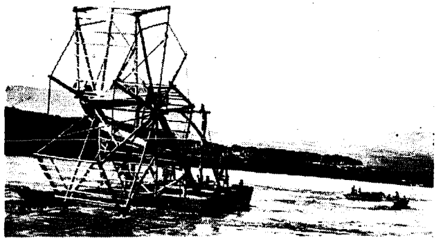
Fig 643 Moving a 'sow' or boat fish wheel, on the Columbia River, Oregon. ( Photo: Donaldson. )
