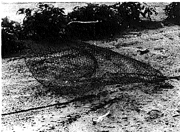
Fig 329 Trap formed of wire mesh without any frame. Lagune Aby, Ivory Coast, (1971).
