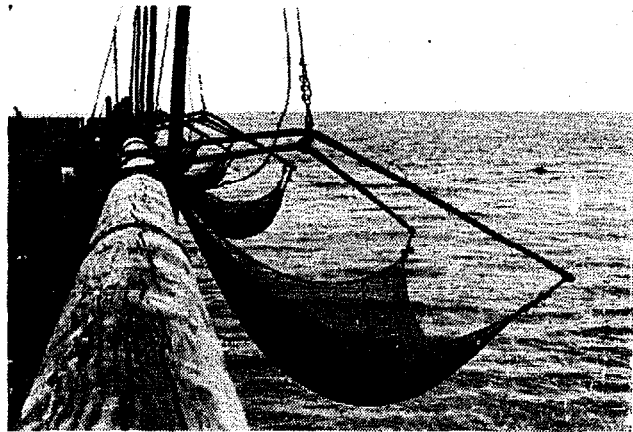
Fig 615 Stationary liftnets to be seen on the harbour mole of Ostend. They can be hired by sports fishermen for bait fishing.
