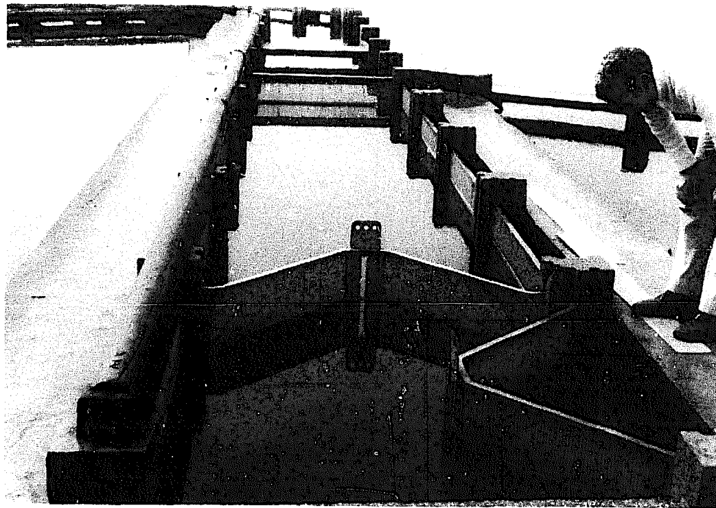
Fig 300 Modern catching chamber in Comacchio (1975).
