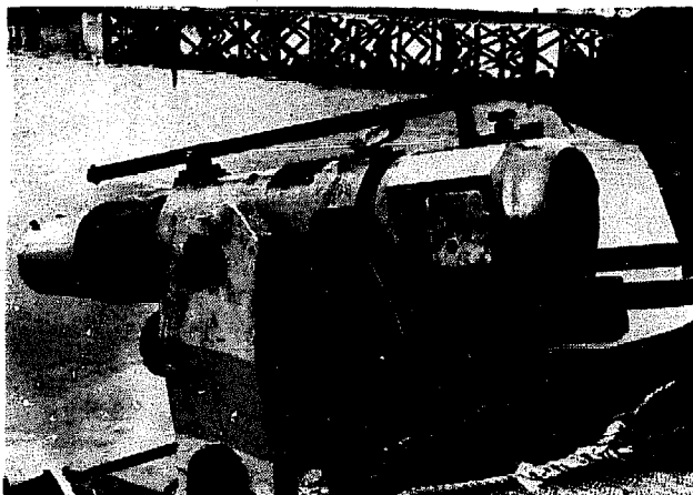
Fig 64 Modern Icelandic whale gun in Reykjavik (1970).
