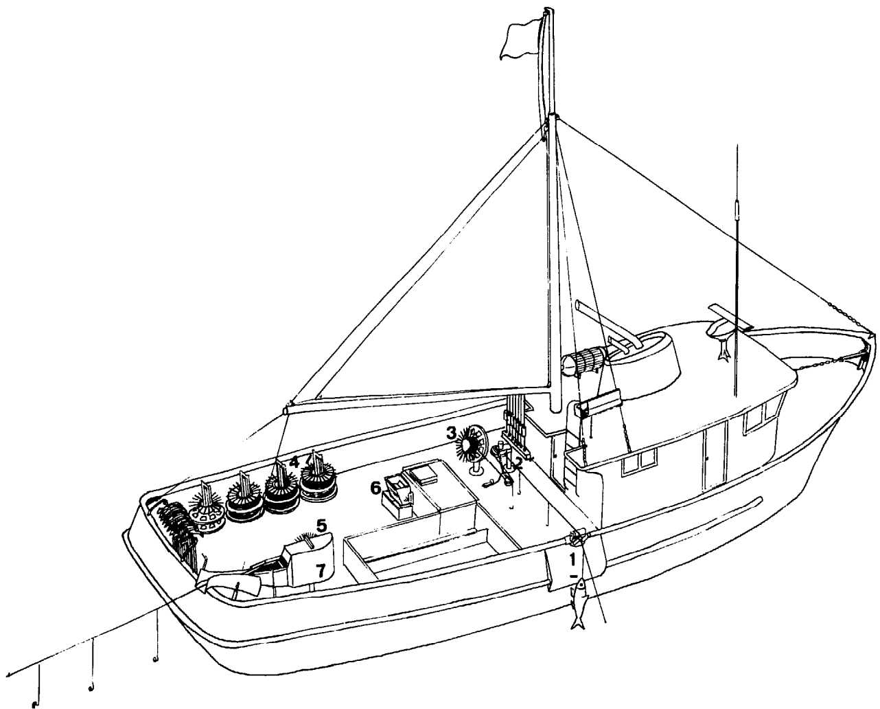
Fig 167 Plan of the deck arrangement for the American Tiler system. (Courtesy of Marco, Seattle, 1978) Hauling the line: (1) adjustable gunwhale roller; (2) line hauler; (3) take-up power head; (4) line storage spools. Setting the line: (5) spool on setting stand; (6) bait-cutting machine; (7) automatic baiter.
