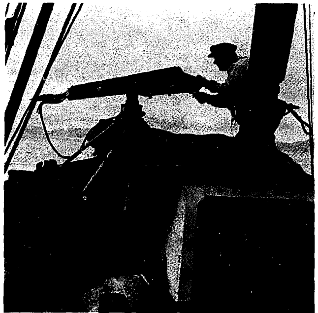
Fig 62 Norwegian harpoon gun for catching small types of whales. (Photo: G Hass, 1942.)
