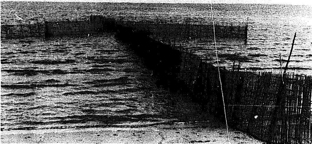
Fig 297 Traplike arrangement of fences in Indonesia. (Photo: Kollmannsperger, 1976.)
