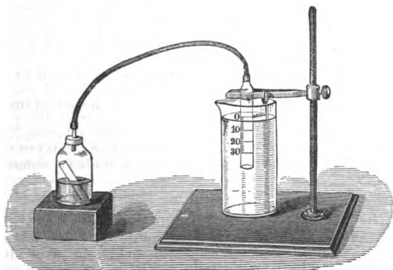
Fig. 63.—Apjohn's Apparatus for the estimation of Urea by the hypo-bromite of sodium solution.
