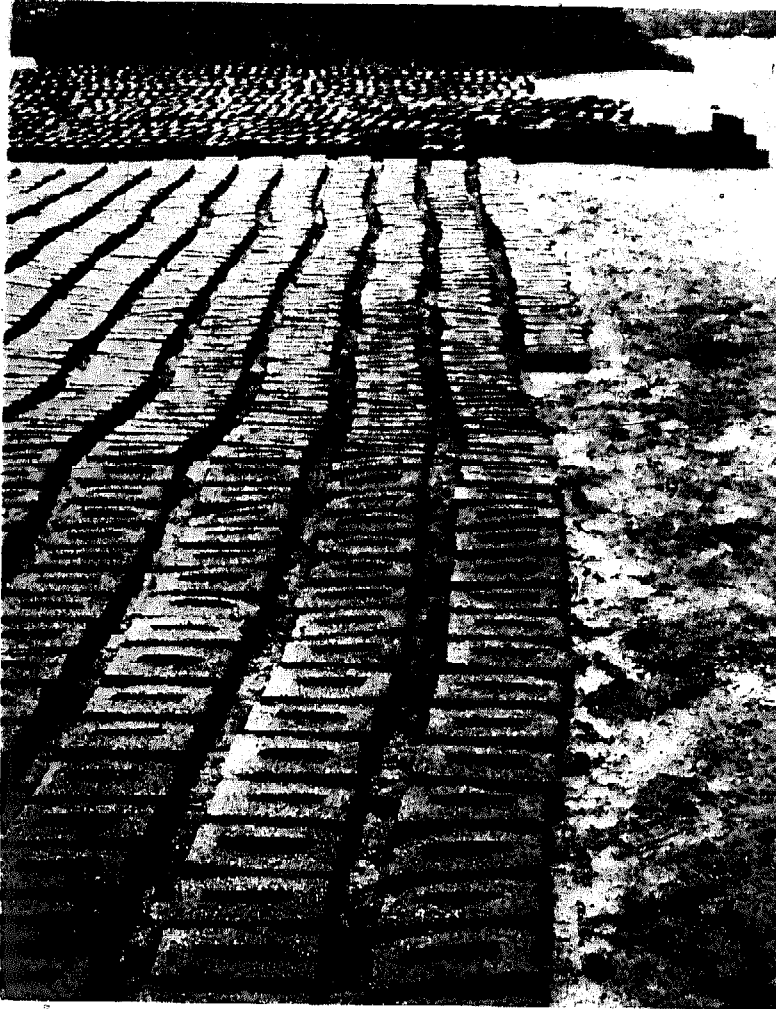
Initially well-shaped slopmoulded bricks with only minor 'flashing' defects subsequently distorted by uneven drying floor
