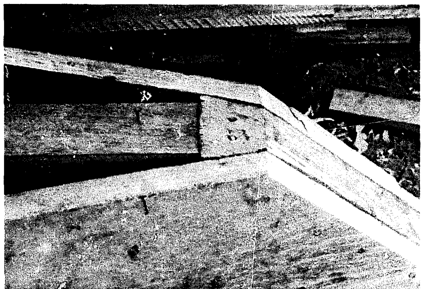
Fig.105 Ajuster le bouchain à effleurer le haut de l'étrave Fig.105 Adjust the chine to be flush with the planed end of the stem
